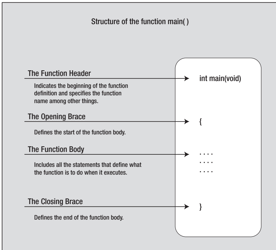
Figure 1-2. Structure of the function main()
